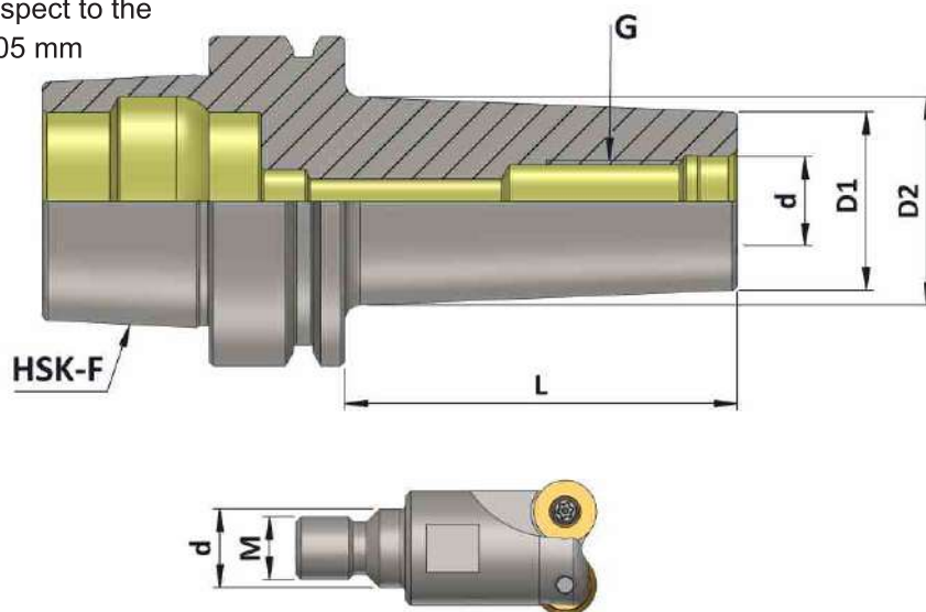
SCREW-TYPE MODULAR MILLING CUTTER
